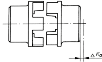
Axial misalignment
